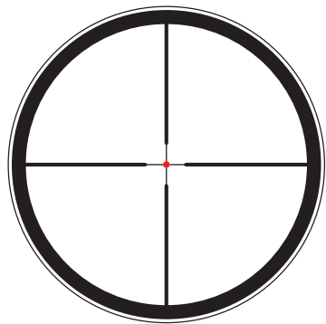
Leica L-Plex reticle (24 mm/42 mm/56 mm)
